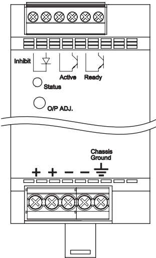
Connector Positions
